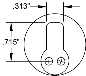
Mortise Cylinder dimensions approximate
