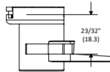
Special milled version for part number RR1250RAILPCSM1
